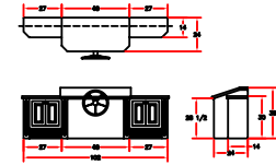
BOAT #001 HELM STATION SCALE: 1/2"=1'-0"
